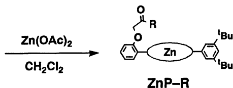
Scheme 3. Synthesis of oligopeptide-linked porphyrins ( ^1\text{AA}=\text{L-amino acid} , ^2\text{AA}=\text{L-amino acid} or L,L-dipeptide, see Ref. 5 for abbreviations).
